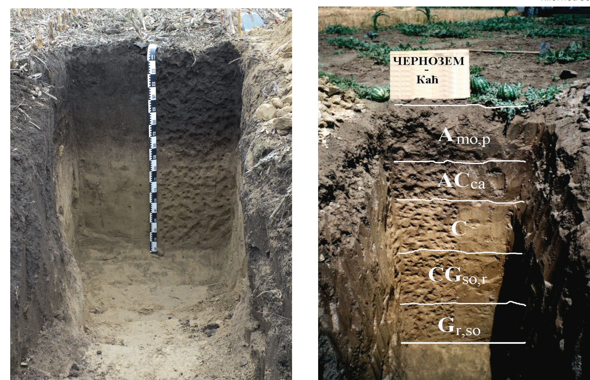
Figure 2. Chernozems in Serbia
